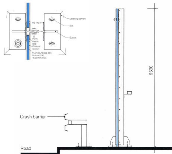
Construction details
